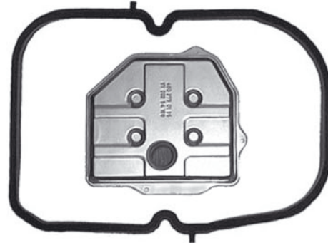
MERCEDES AMBULANCE Pan Gasket MERC126.GAS01 Filter MERC126.FIL03 25mm Pick Up
