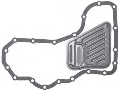
FORD AX4N Pan Gasket AX4N.GAS11 Filter AXODE.FIL02 Filter has Orange Seal
