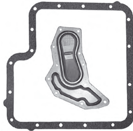
FORD C6 Pan Gasket C6.GAS01 Filter C6.FIL02
