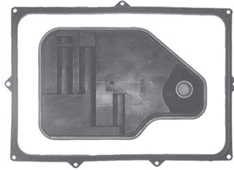
BTR 74LE Pan Gasket BTR74.GAS01 Filter BTR74.FIL01 Neck 22.4mm High
