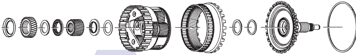
Rear Planetary and Output
