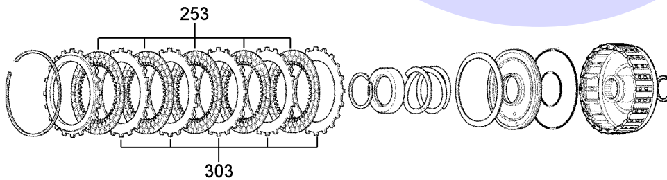
Secondary Shaft, First & SEcond Clutches
