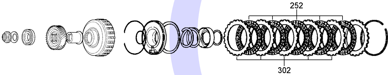
Countershaft
