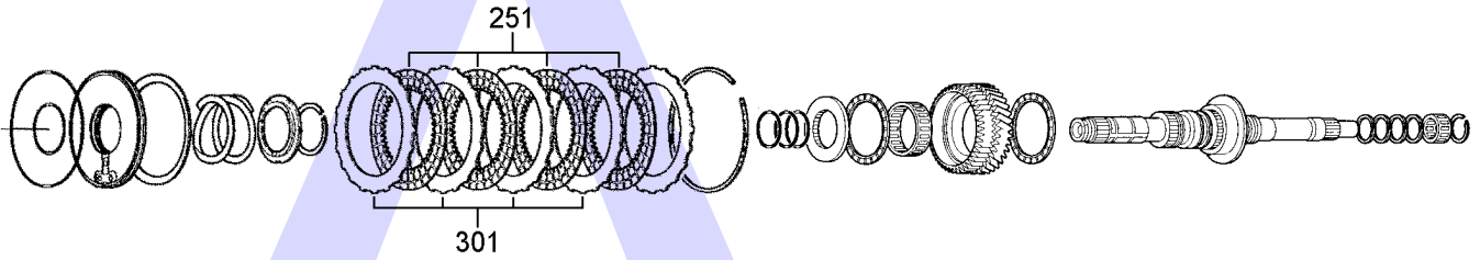
Mainshaft, Third & Fourth Clutches
