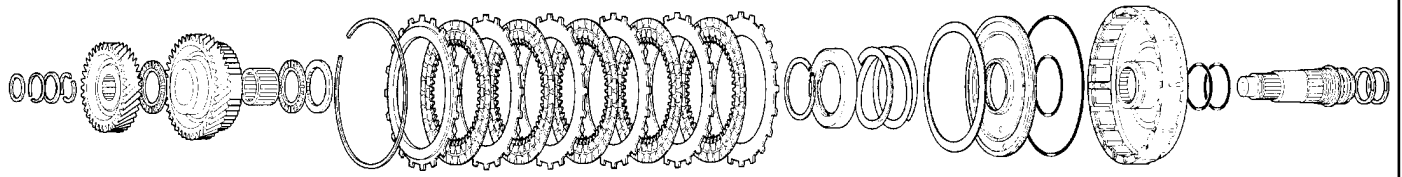
Intermediary Shaft & Third Clutch
