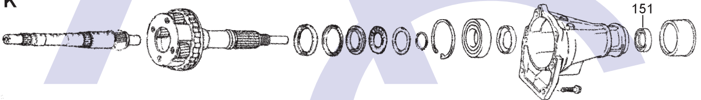
REAR PLANETARY ASSEMBLY
