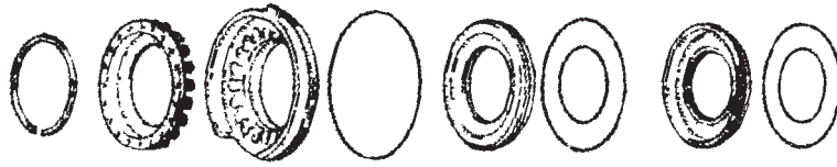
B4 (LOW & REVERSE) BRAKE PISTON ASSEMBLY
