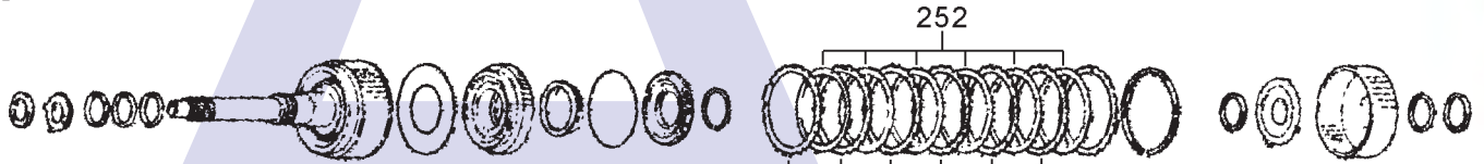
'C1' (Forward) Clutch
