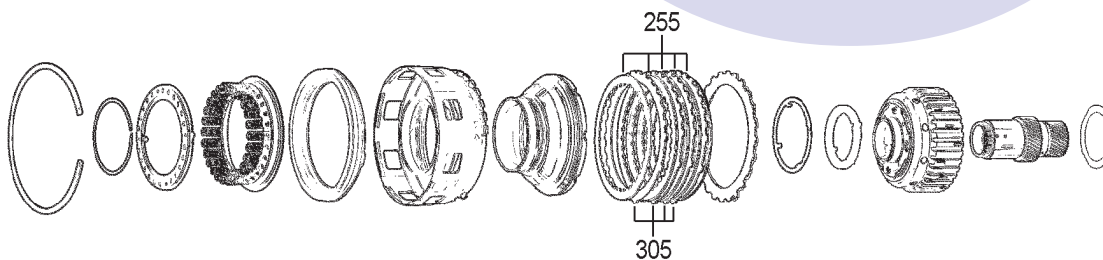
Third Brake
