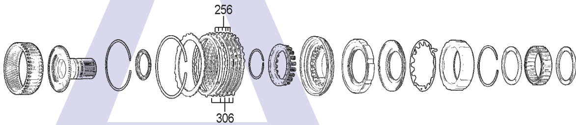
Low/Reverse Brake
