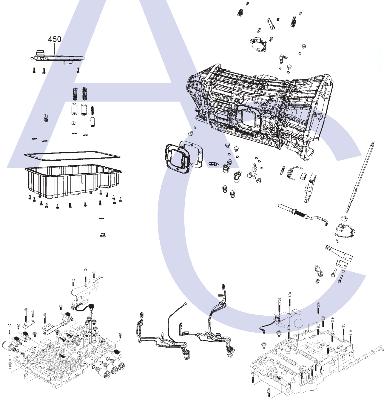
Casings, Oil Pan, External Components, Valve Body Etc
