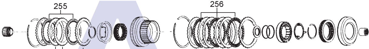
Overdrive Direct Clutch
