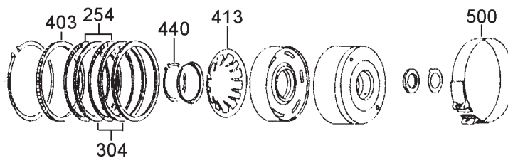
Reverse Clutch & 2-4 Band
