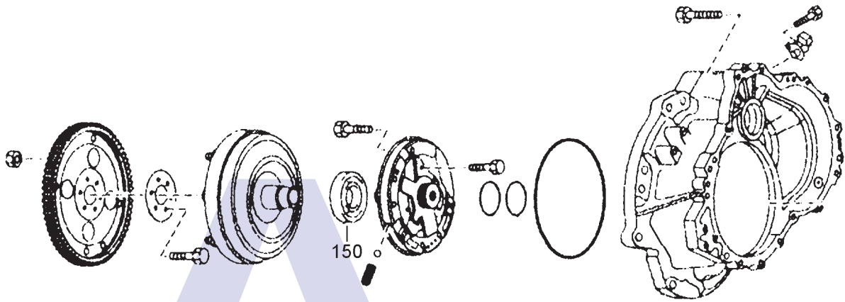
Converter, Pump & Bell Housing
