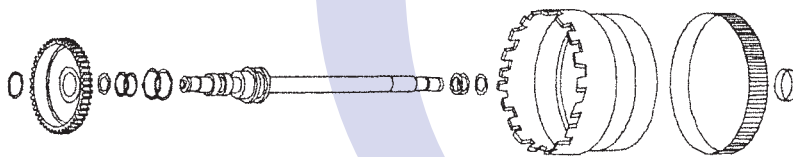
'C1' Hub and 'C2' Cylinder
