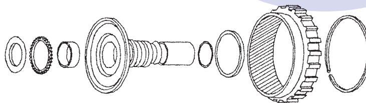
Output Shaft and Rear Annulus
