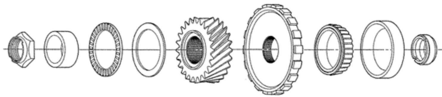
Front Differential Transfer Drive Gear Assy
