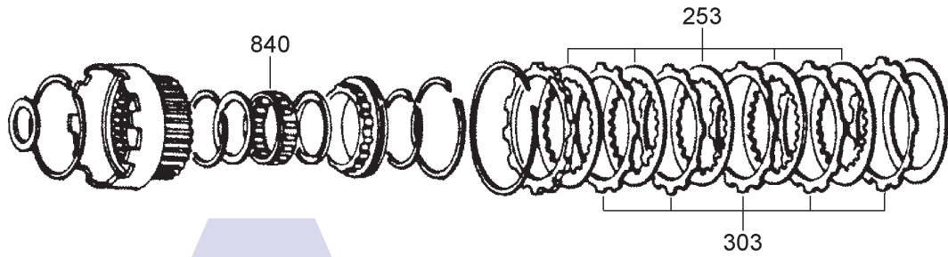
LOW REVERSE BRAKE
